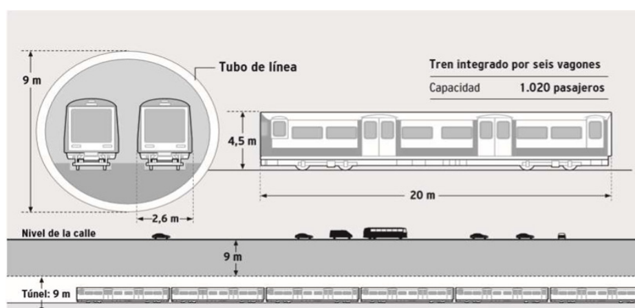
Figure 13. Characteristics of the Córdoba Underground
