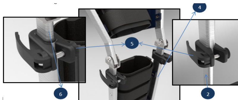
Figure 32. Height adjustment
