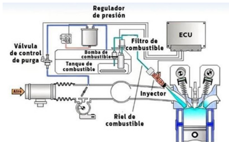
Figure 4. General representation of a fuel system
