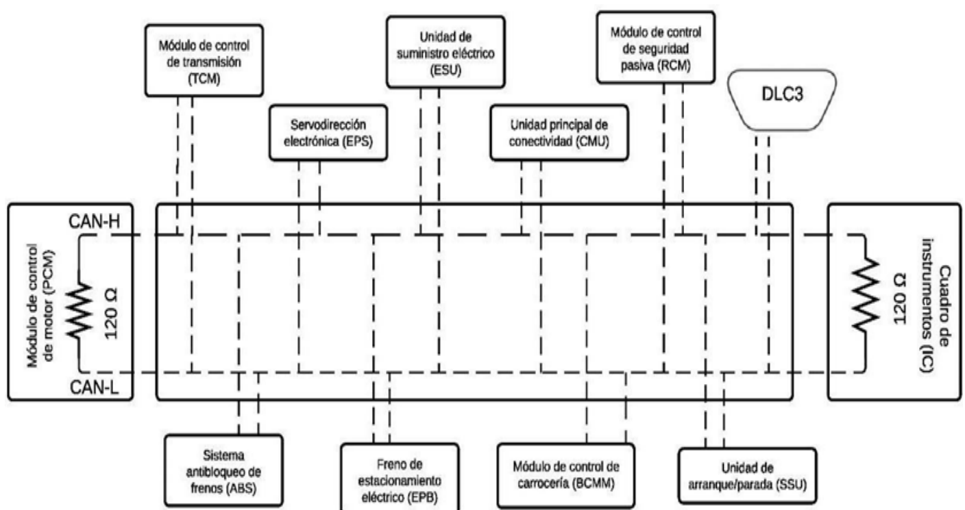
Figure 5. CAN bus (500 kbps) of the 2019 Mazda CX-3 vehicle
