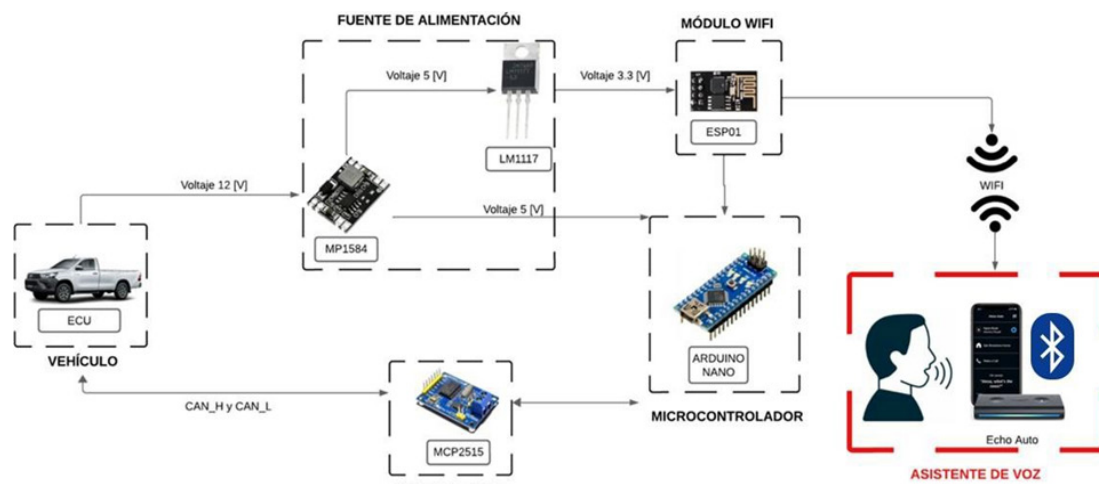
Figure 1. Block diagram of the hardware for interconnecting the vehicle computer and Alexa Auto
