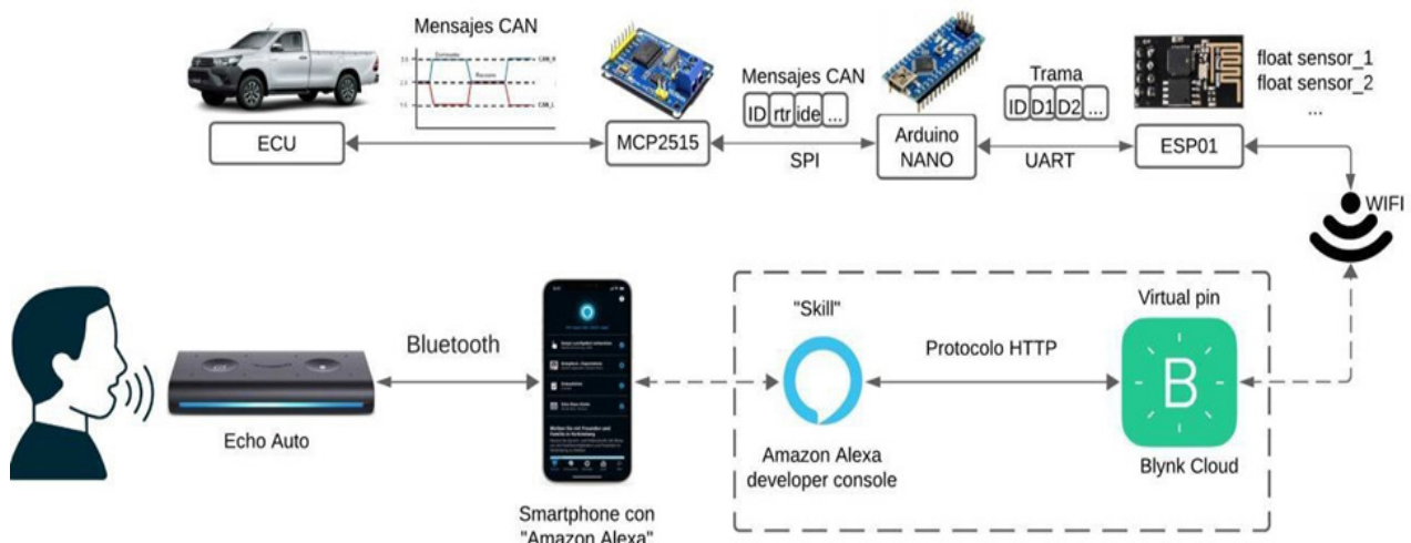
Figure 17. Diagram for interconnection of Alexa Auto and the vehicle computer
