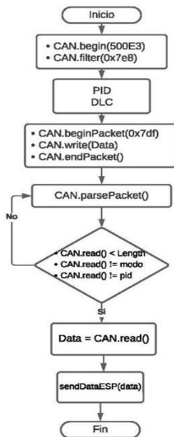
Figure 9. Flowchart for reading ECU sensor information using Arduino Nano
